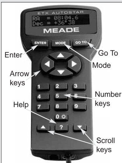
Fig. 21: AutoStar keys.
