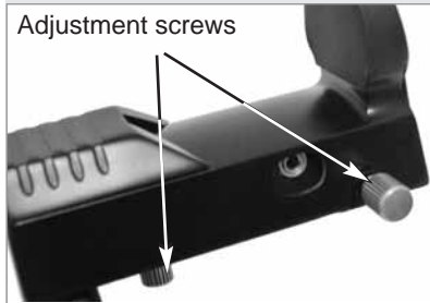
Fig. 54: The LNT Module, with adjustment screws and Atomic Time Update port visible.
