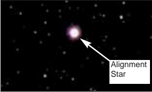
Fig. 25: During alignment, the alignment star is always the brightest star in the area of the sky at which the telescope is pointing.
