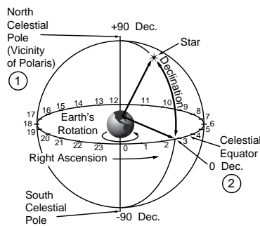
Fig. 43: Celestial Sphere.
