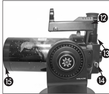
Fig. 15: Insert eyepiece.
