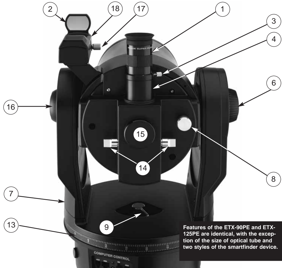
Fig. 1b: Rear View
