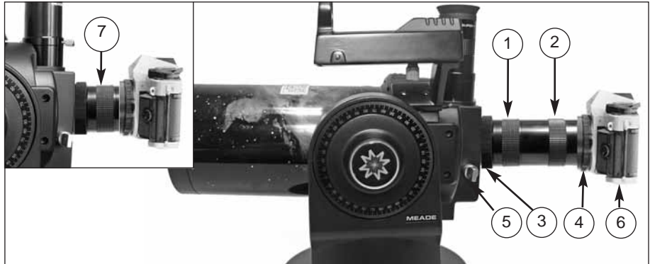
Fig. 30: Example of photography through the ETX using the #64 T-Adapter: (1) Short section of #64 T-Adapter; (2) Extension section of #64 T-Adapter; (3) Knurled attachment ring; (4) T-mount; (5) Flip-mirror control in “up” position; (6) 35mm camera body; (7) Format 1.
