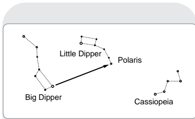
Fig. 50: Locating Polaris
