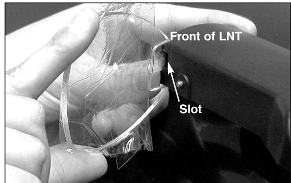
Fig. C: Inset tongue into LNT module slot.
