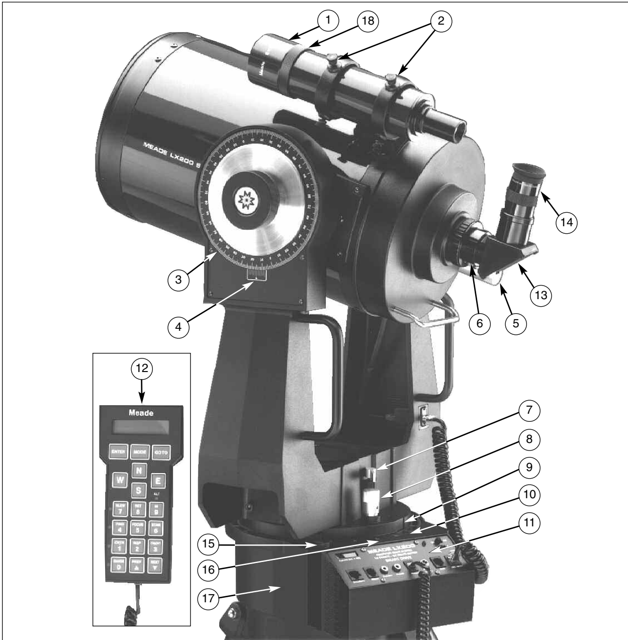
Fig. 1: 8" LX200 Telescope.
