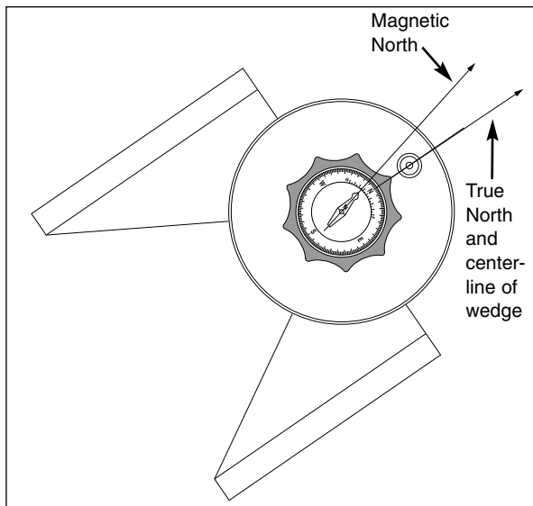
Fig. 19: Equatorial Wedge.
