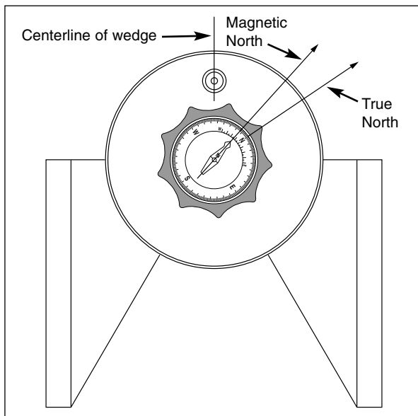
Fig. 18: Equatorial Wedge.
