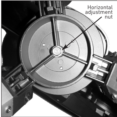
Fig. 7: Horizontal adjustment nut. (View of the underside of the base.)
