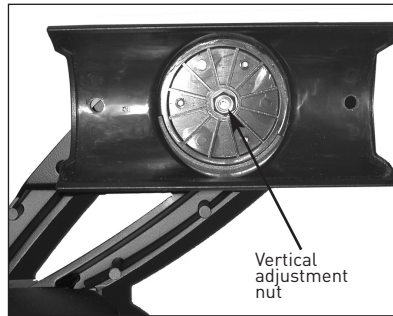
Fig. 8: Vertical adjustment nut. (Bracket shown with optical tube removed.)
